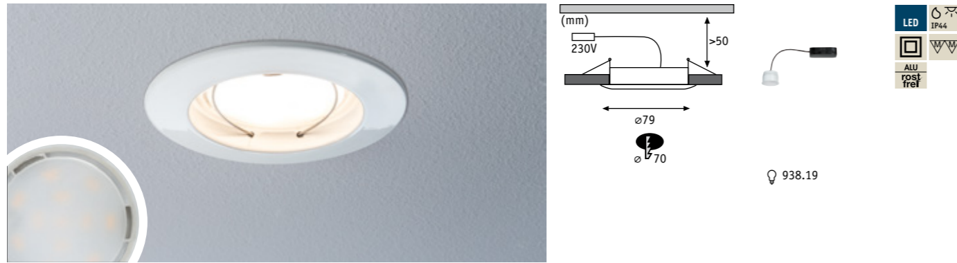
Premium Line LED 230V Coin 51mm Hliník zinek Aluminium Cynk Aluminiy Цинк
