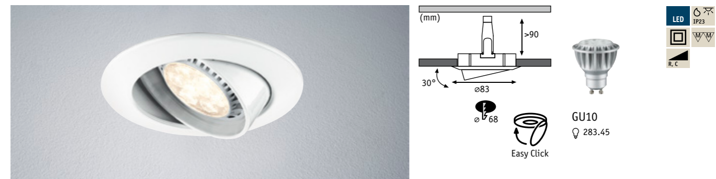
Premium Line Power LED 230V GU10 51mm
